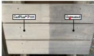
Test Rig, Accoya Technical Centre, Arnhem, the Netherlands 12 months weathering. South facing cladding panels
